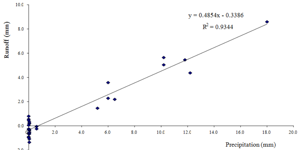
Figure 6: Effects of Precipitation on Runoff
