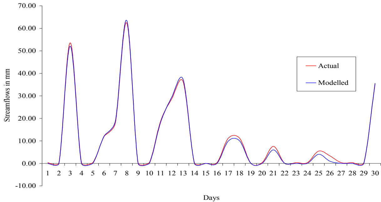
Figure 3: September Actual and Modelled Streamflows
