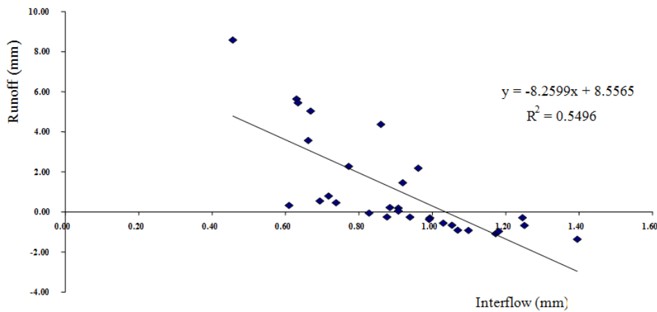
Figure 8: Effects of Interflow on Runoff
