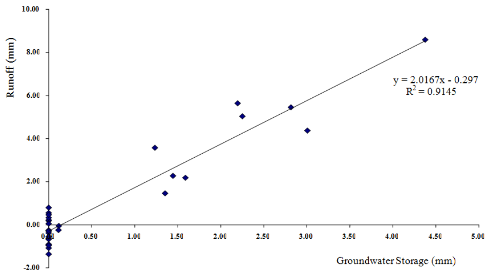
Figure 7: Effects of Groundwater Storage on Runoff
