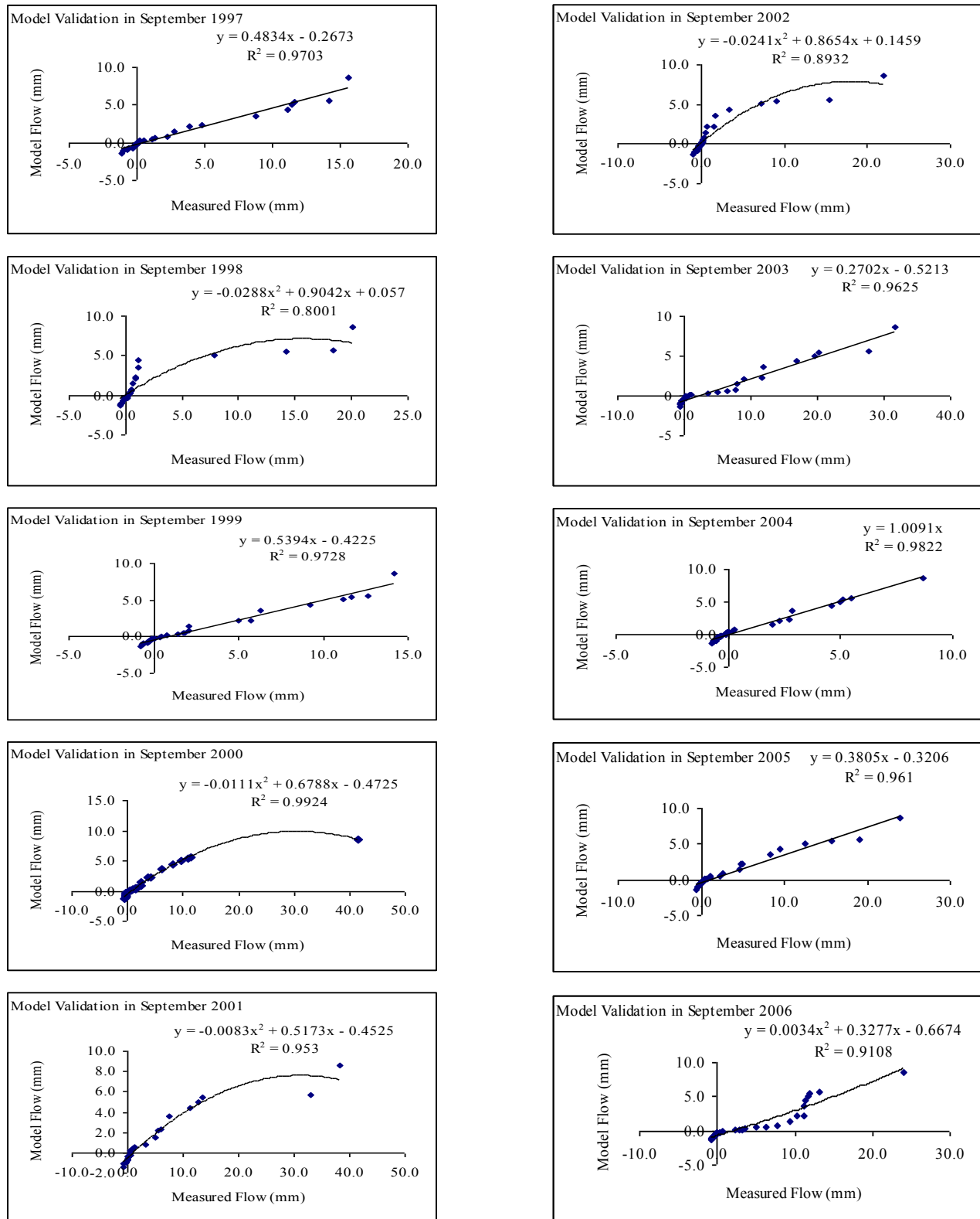
Figure 4: September Model Validation
